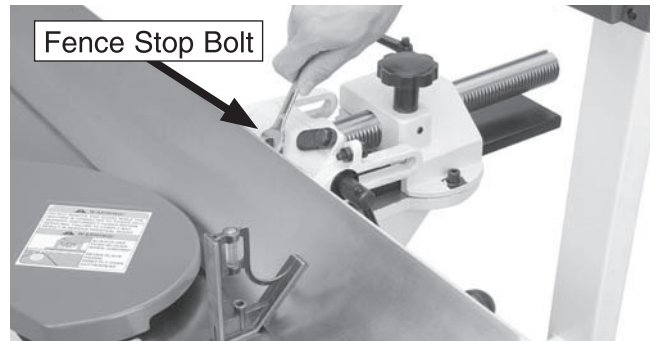
45° outward fence stop jam nut
