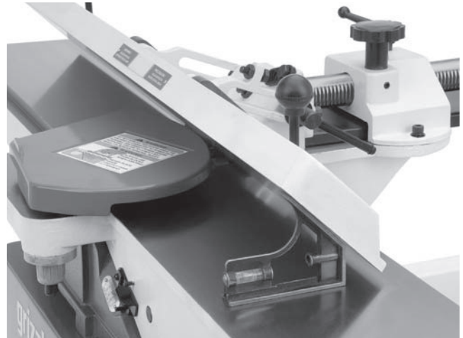
Adjusting fence 45° inward.
