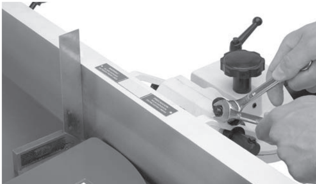
90° swing stop engaged.
